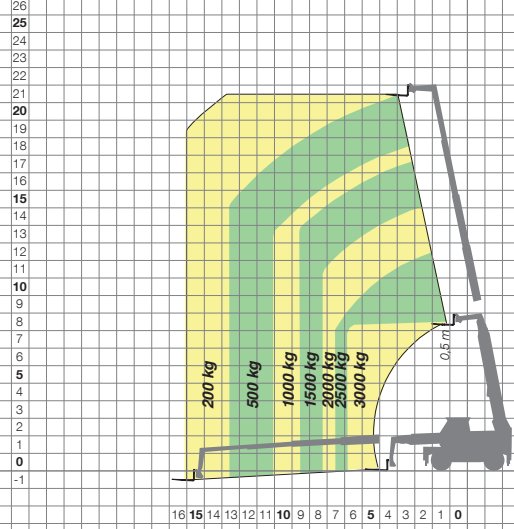
ROTO 40-26 MCSS FORKS ON TYRES - FRONT
