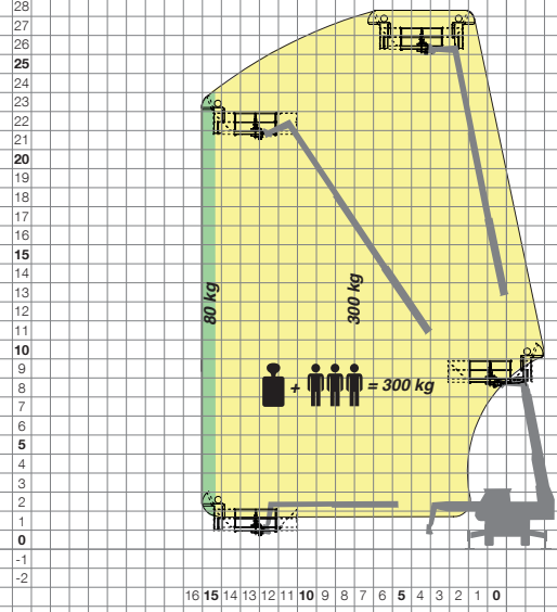
ROTO 40-26 MCSS AERIAL WORK PLATFORM THROUGH 360°
