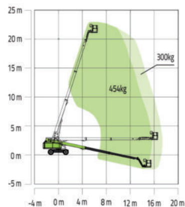
ZT20J Working Envelope
